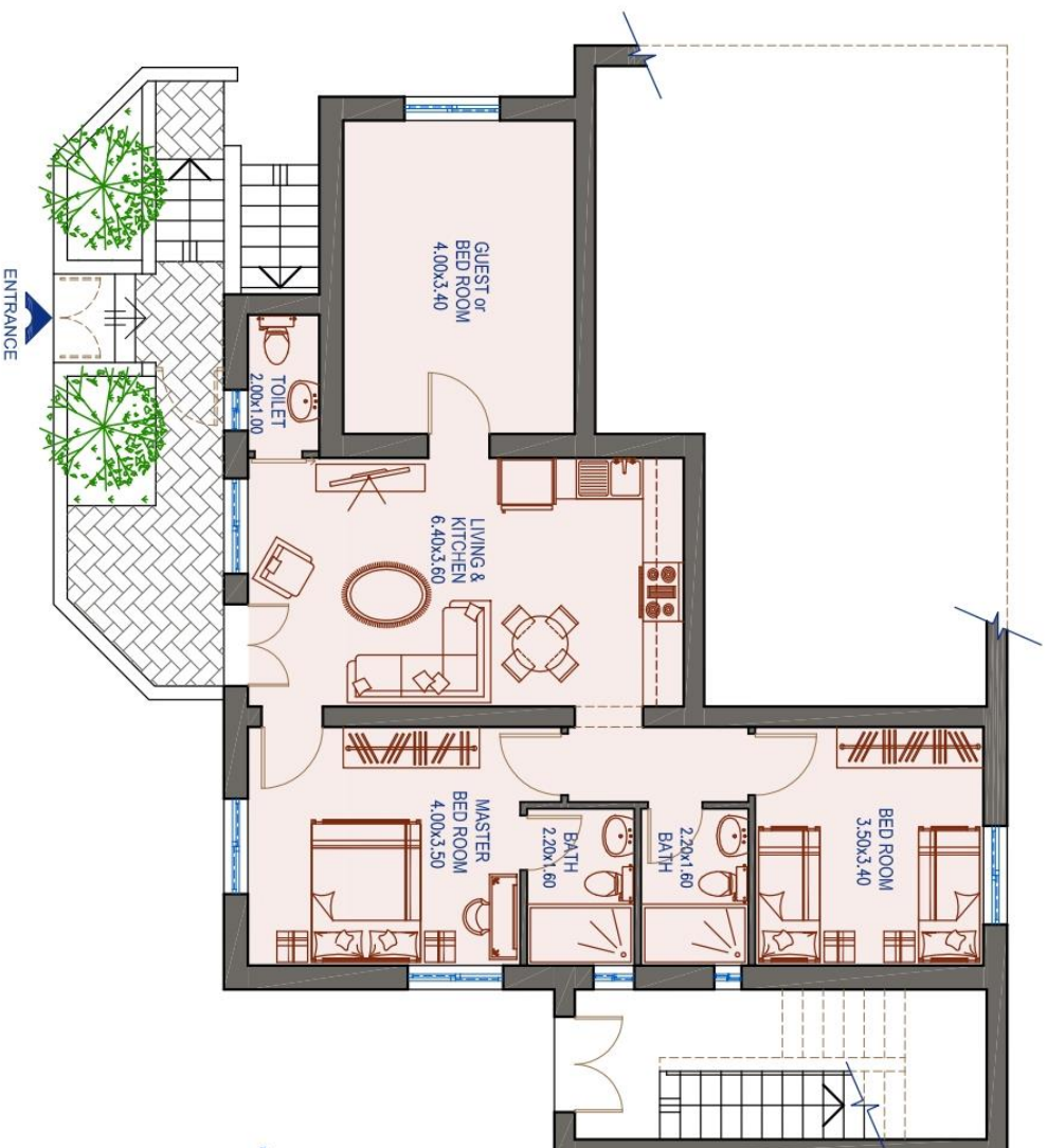
1st Floor
